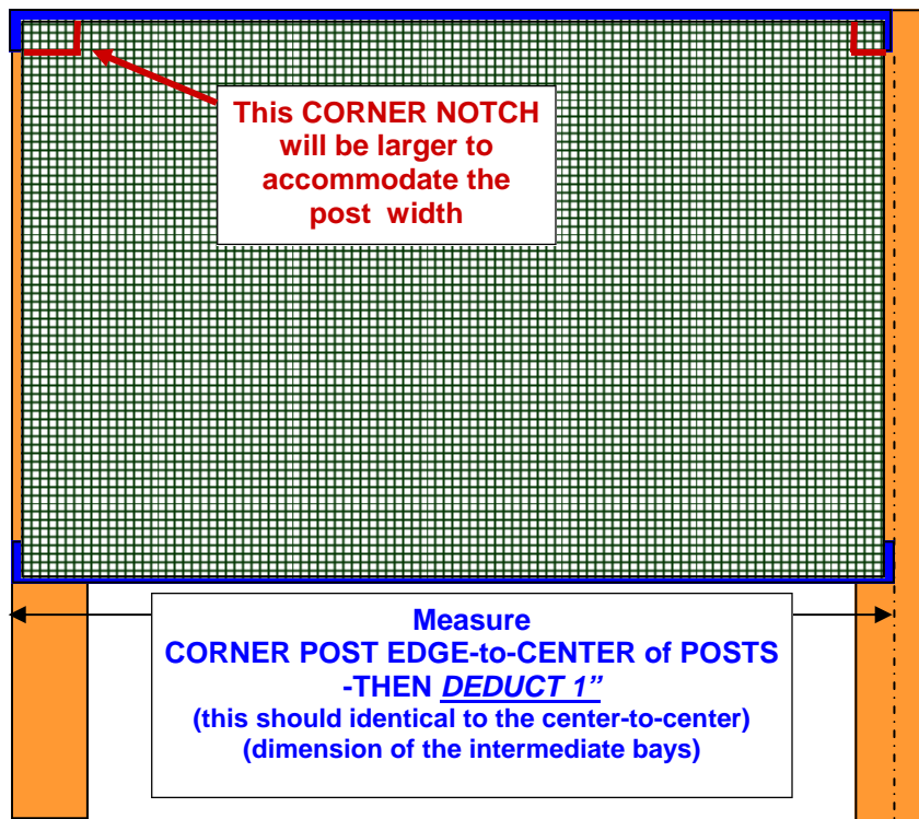
CORNER BAY - FRONT VIEW
